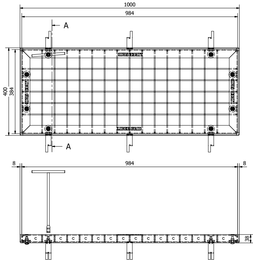
DETAIL 1
